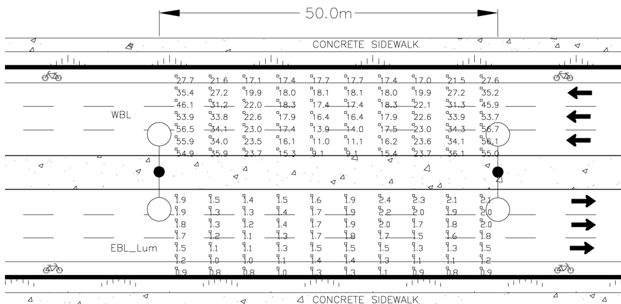
Figure 7.2 Roadway Lighting Design Using Luminance &amp; Illuminance
