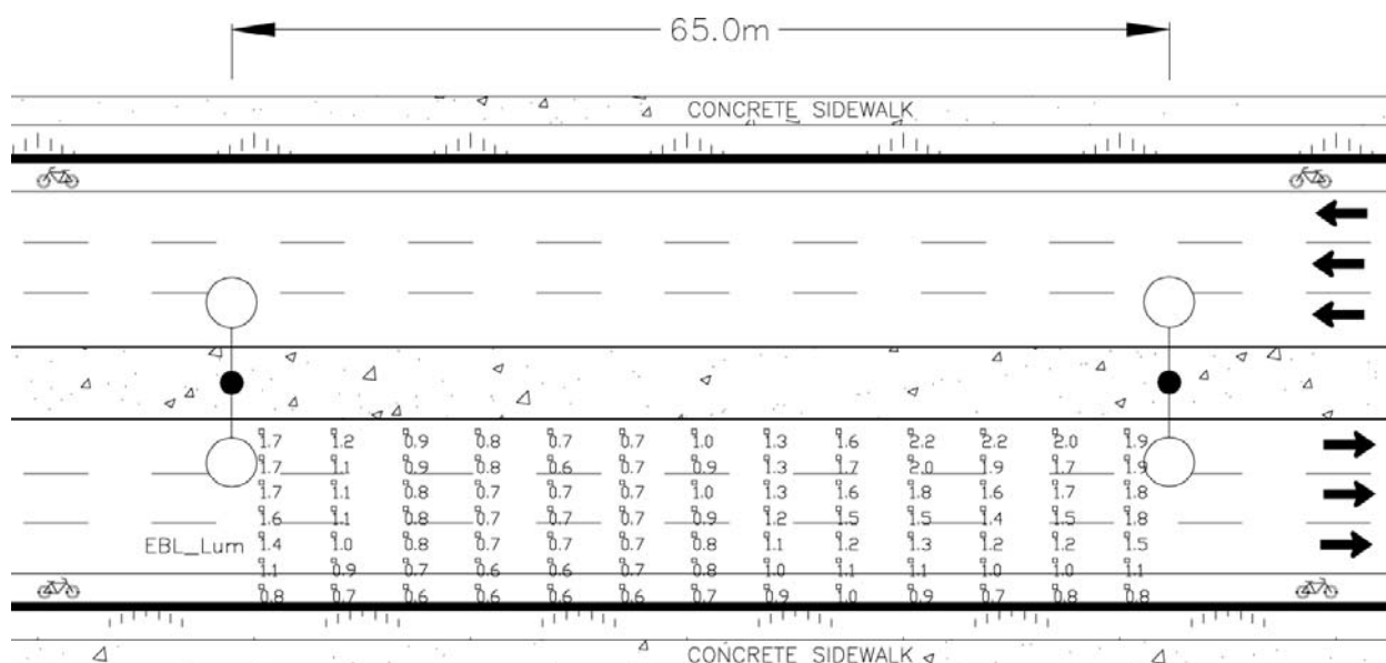
Figure 7.1 Roadway Lighting Design Using Luminance
