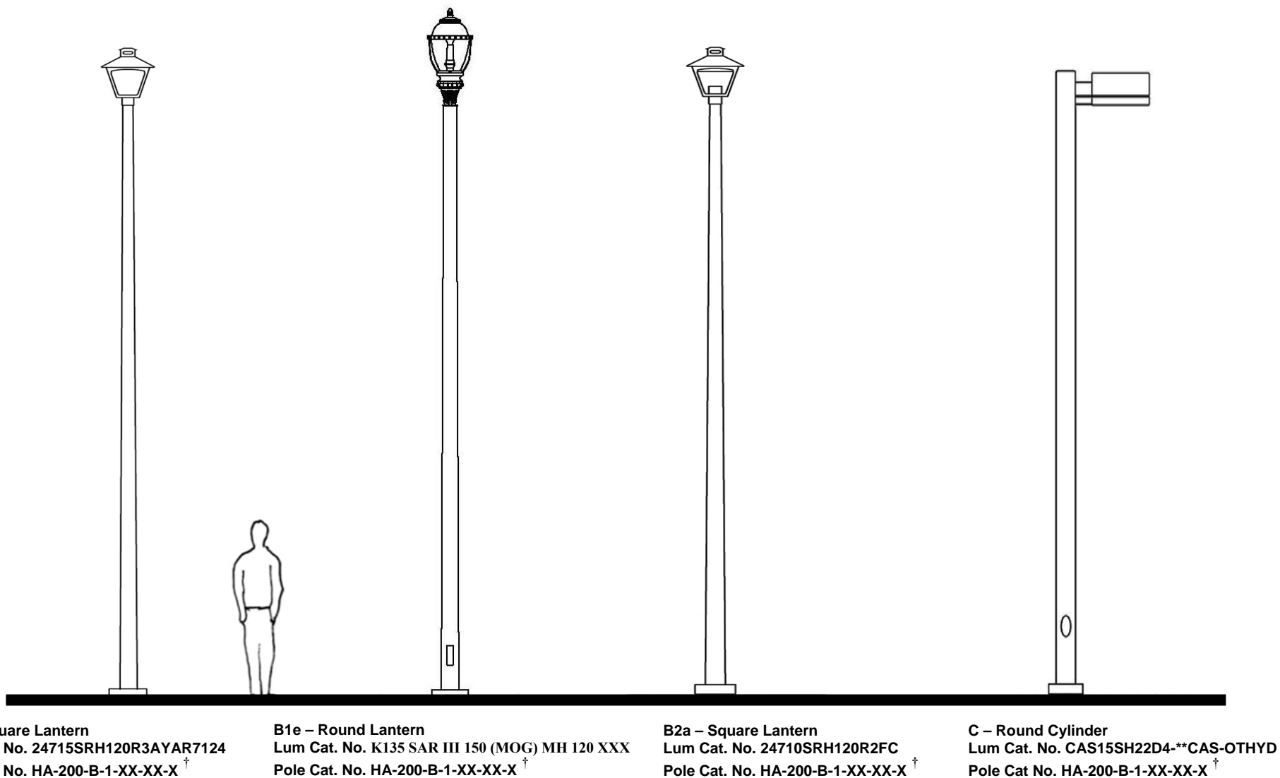
Figure 5.7 Decorative Lighting Assemblies for 'Mid-Height' Poles
